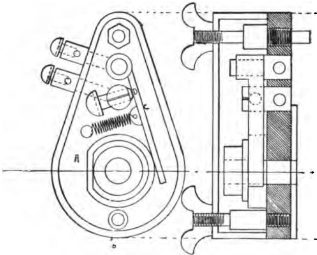
FIG. 335.--The "Dyke" Contact Breaker, shown in plan and part vertical section. Unlike the De Dion contact breaker, the cam, A , has no notch, but is flattened at one point on its circumference, so that the trembler spring, C , is periodically brought into contact with the other terminal of the circuit with the minimum of wear and shock. The advantages claimed for this device are consequent superior durability and quite as good effect in making and breaking primary circuit.
